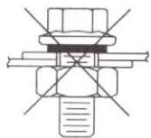
Figure 31. Bolt Torque Illustrations
